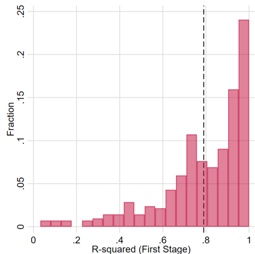
Figure SA-H.1. R-squared Distribution in the Estimation of the Tariff Function
