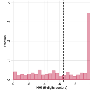
Figure SA-A.3. Distribution of Herfindahl-Hirschman Indices for Manufacturing in 2017
