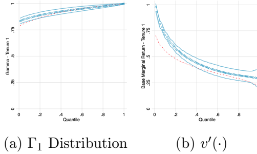
Figure SA-F.3. Monte Carlo Results for Tenure 1
