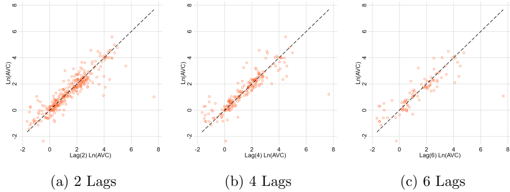
Figure SA-G.1. Serial Correlation
