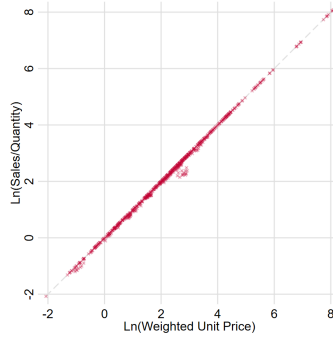
Figure SA-A.1. Average Price vs Weighted Price
