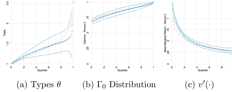
Figure SA-F.2. Monte Carlo Results for Tenure 0
