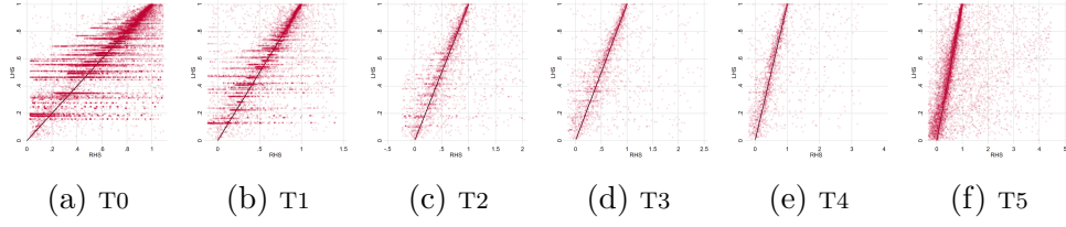
Figure SA-H.4. Model Fit - Statistical
