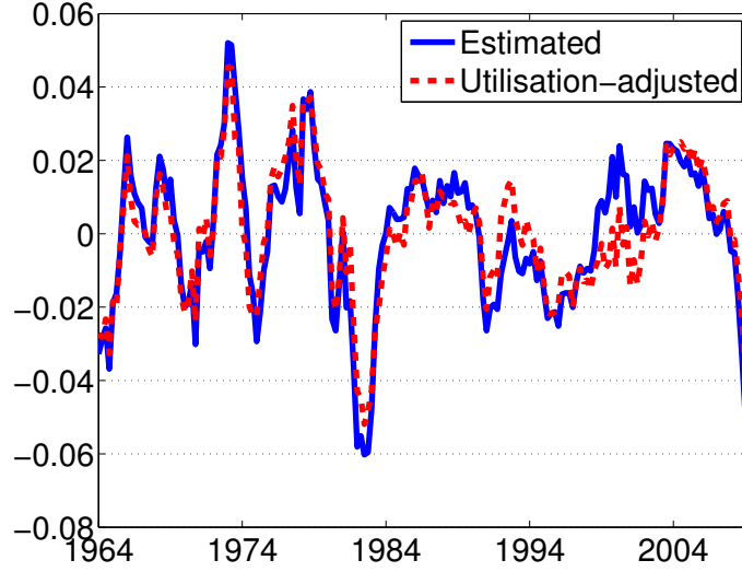
Figure A1: Estimated technology and utilization-adjusted technology in US data, 1964–2009
