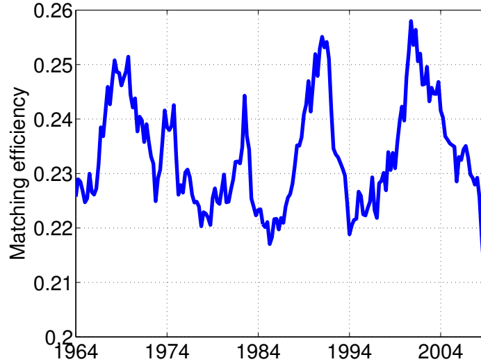
Figure A2: Matching efficiency in US data, 1964–2009
