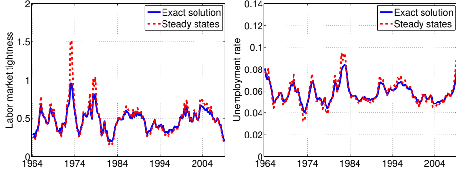
Figure A11: Labor market tightness and unemployment across solution methods.
