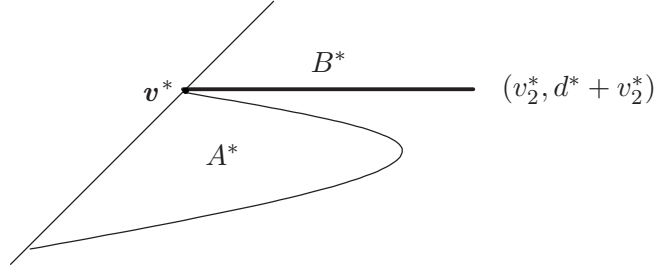
FIGURE 2. SETS A^* AND B^* IN CASE 1
