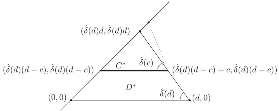
FIGURE 1. SETS C^* AND D^* IN STEP 2 OF LEMMA 9
