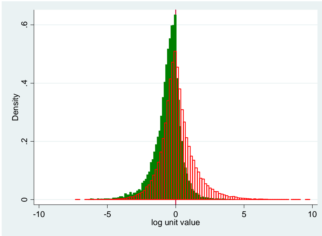
Appendix Figure 1- Distributions of unit values by distance
